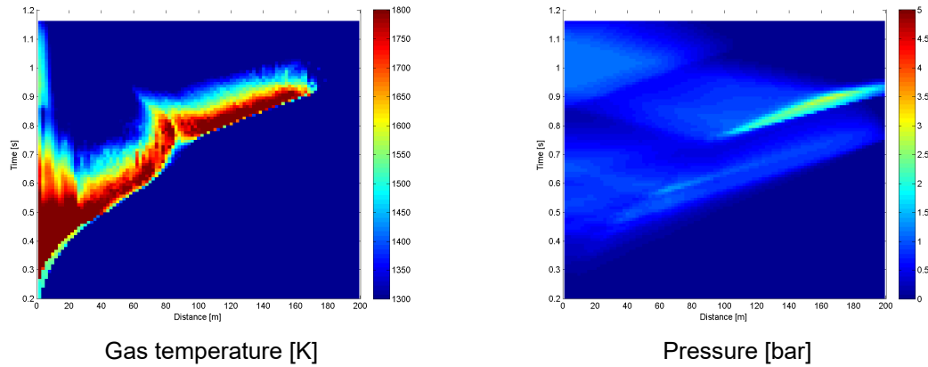
Figure 4-2 Simulated 'Double Strong' explosion results
