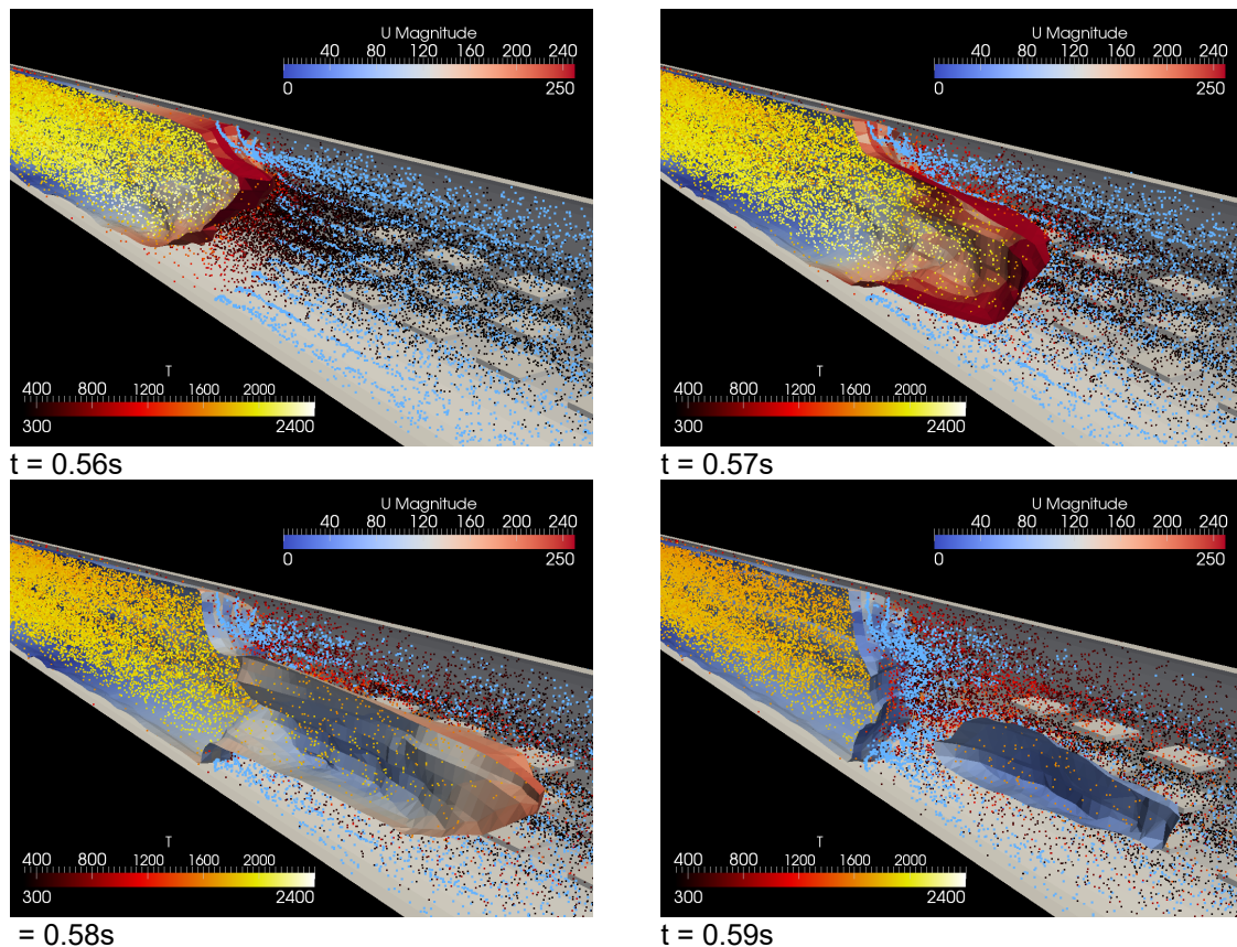
Figure 4-3 Initial active barrier concept.
