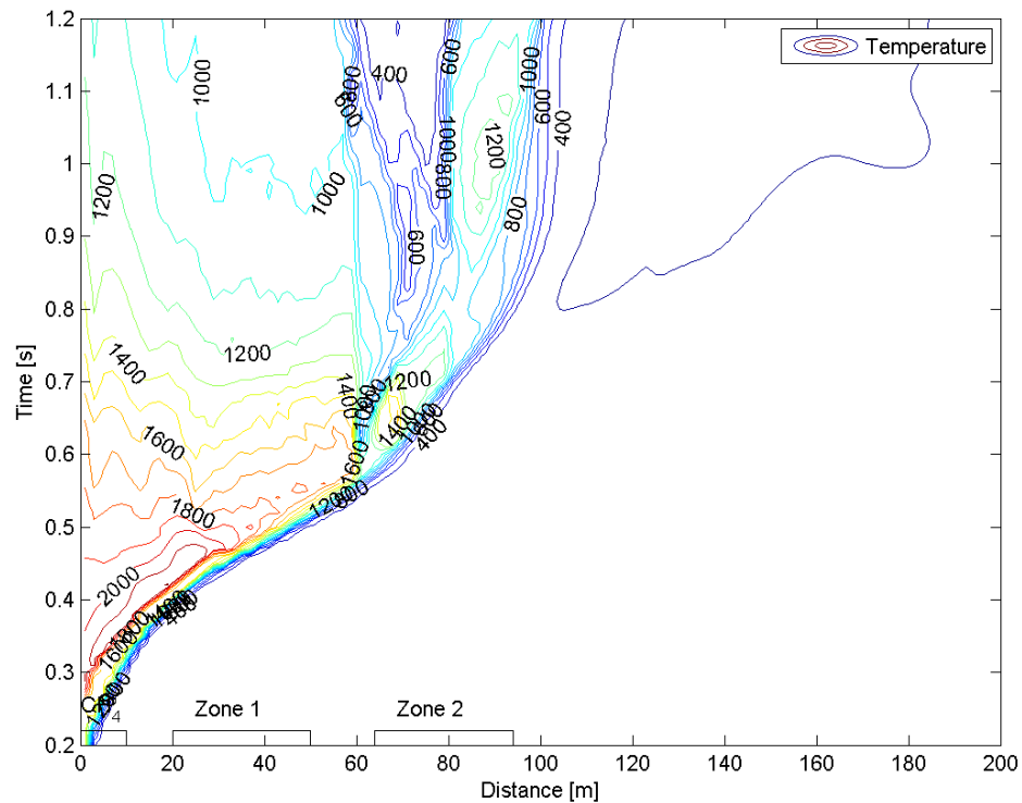
Figure 4-5 Triple ring, 100 µm droplets, 200 l/s flowrate.
