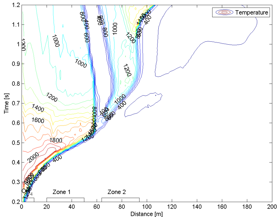
Figure 4-4 Single ring, 20 \mu\text{m} droplets, 200 l/s flowrate.
