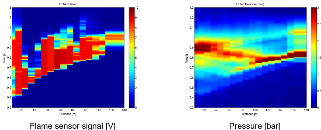
Figure 4-1 Typical ‘Double Strong’ test results
