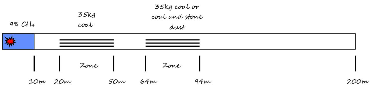
Figure 2-2 Kloppersbos tunnel layout – double strong coal dust explosion (not to scale)
