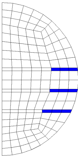
Figure 3-1 Klopersbos tunnel CFD mesh cross-section
